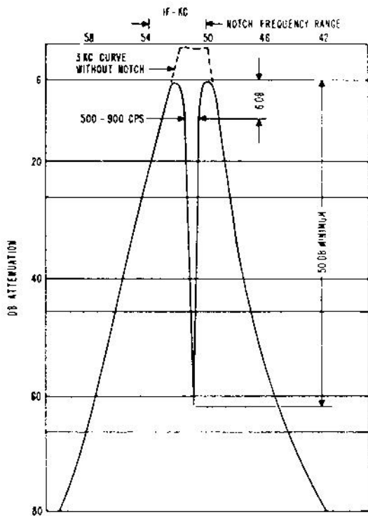
Figure 8. IF Selectivity Curve with Notch
